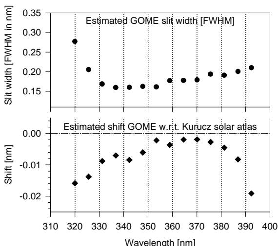
Figure 1. Shift and slit width parameters derived from non-linear least-squares fitting between a GOME solar irradiance and the high-resolution Kurucz atlas (see text).
